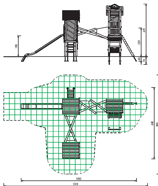
5 66 267 5 elbe ibondo play system Alamo1:200
