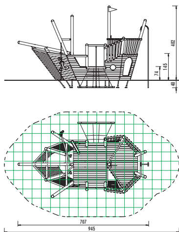
5 59 146 5 elbe tema Sand Ship Nina 1:200
