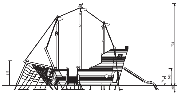
5 59 151 5 eibe tema play ship Santa Maria 1:200
