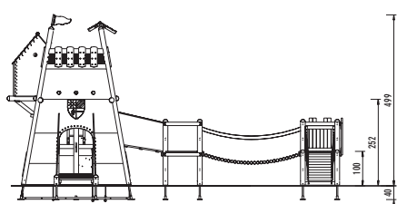
5 66 360 5 eibe tema Castle Tower 1:200
