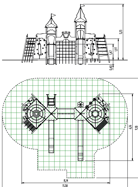
5 66 572 0 elbe ibondo play system Cristal 1:200
