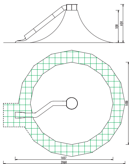
5 51 850 0 eibe tema Iceberg with Toboggan Run 1:300
